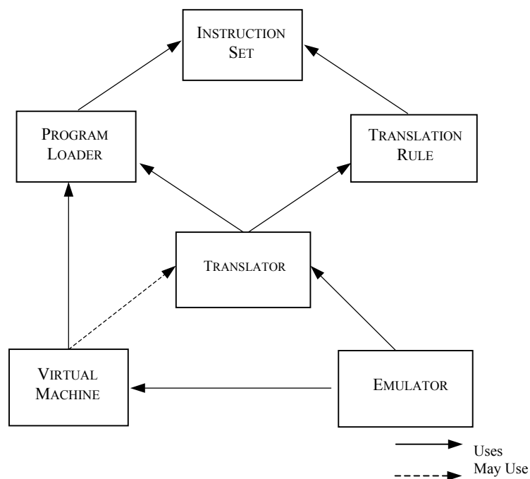
Figure 17. The roadmap of the EXTREM-COMPILING pattern language
