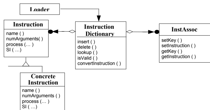
Figure 11. The INSTRUCTION-SET pattern (structure)
